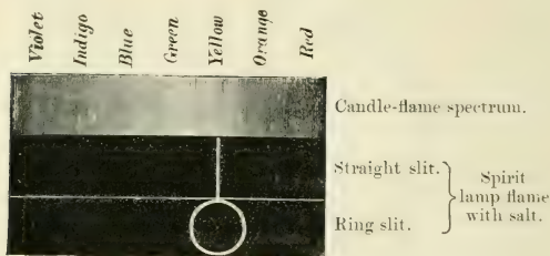
FIG. 3.—A continuous and a discontinuous spectrum.
